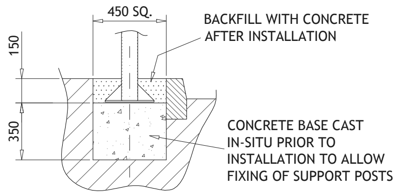
OPTIONAL POST FIXING DETAIL
